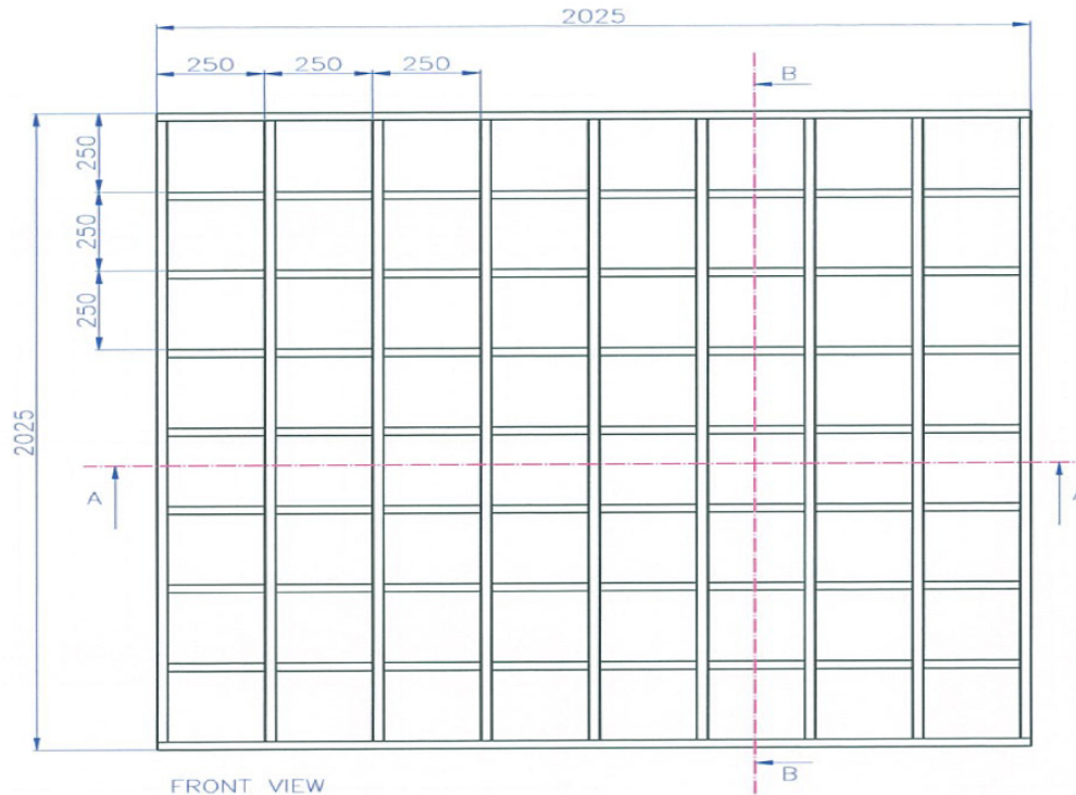
FRONT VIEW
