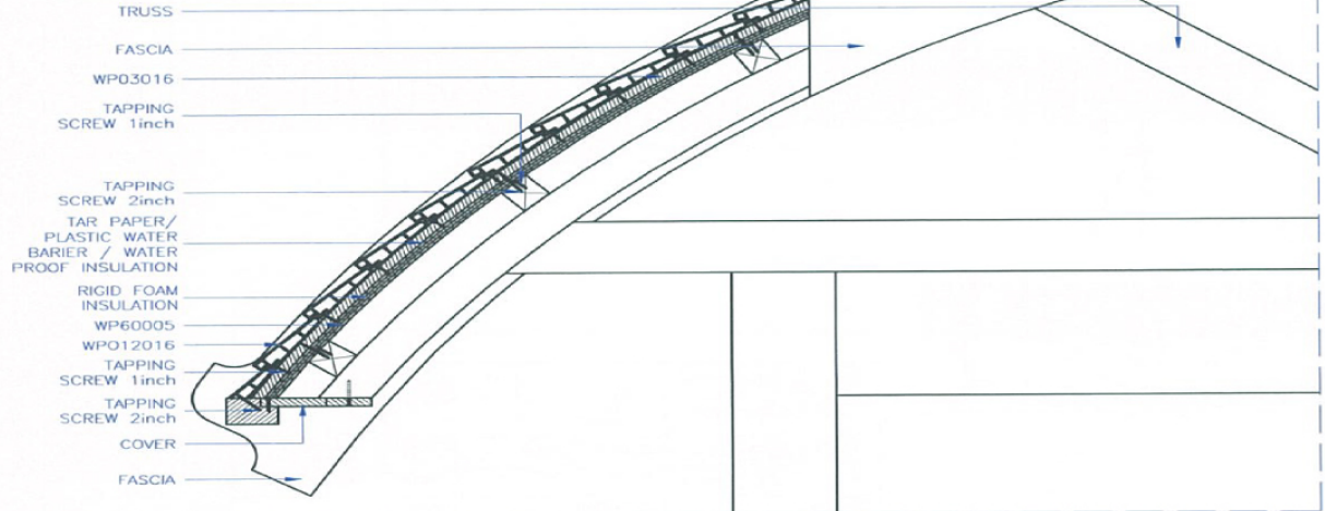
DETAIL B
