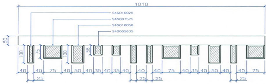
TOP VIEW
