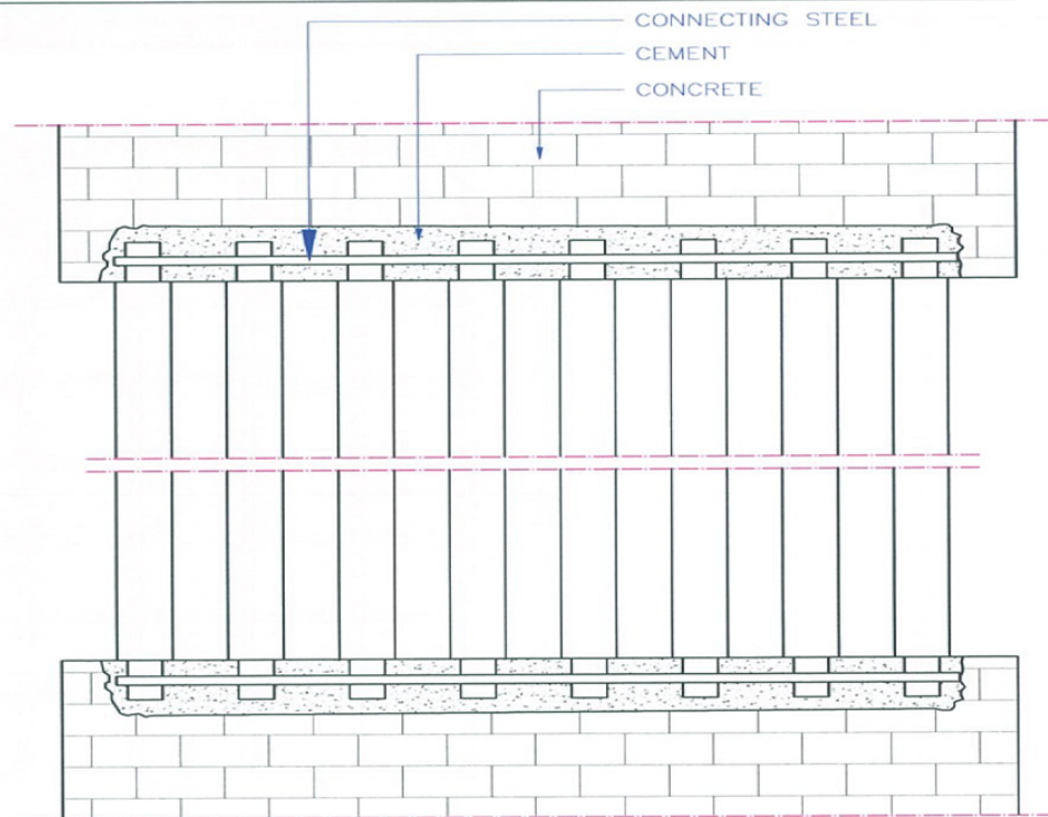
FRONT VIEW
