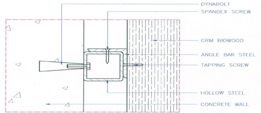
DETAIL
