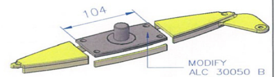
COVER, IF12508
