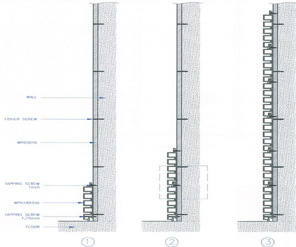
SIDE VIEW
