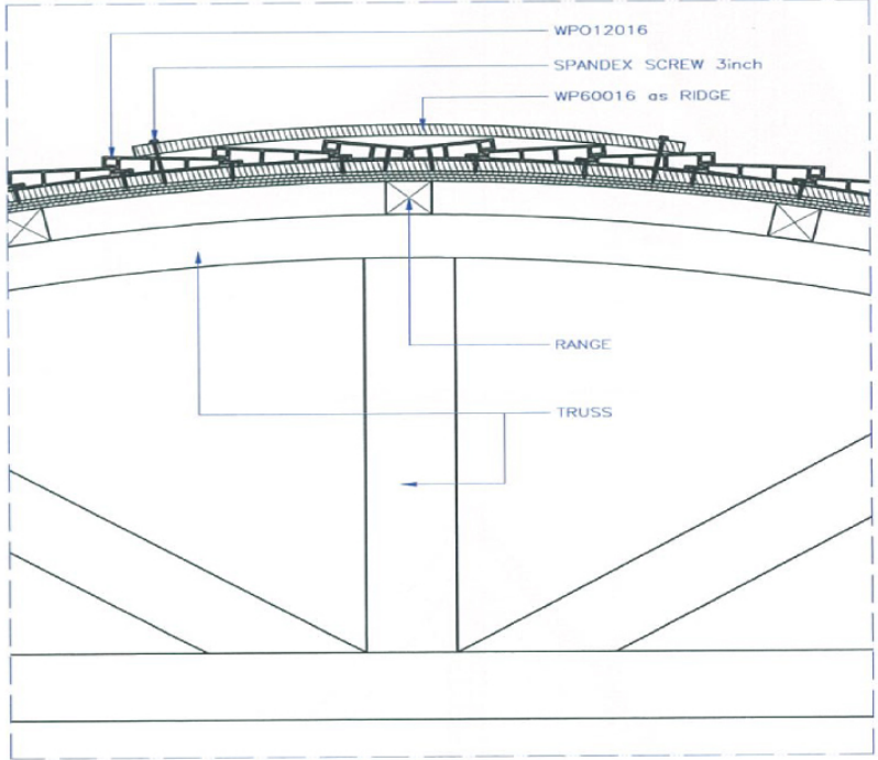
DETAIL A
