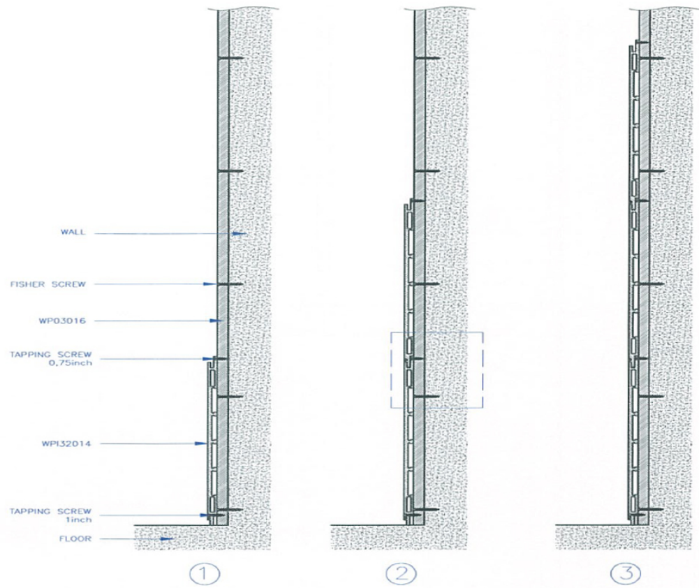
SIDE VIEW
