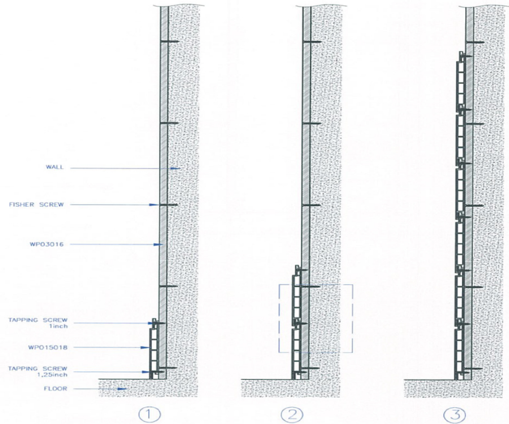
SIDE VIEW
