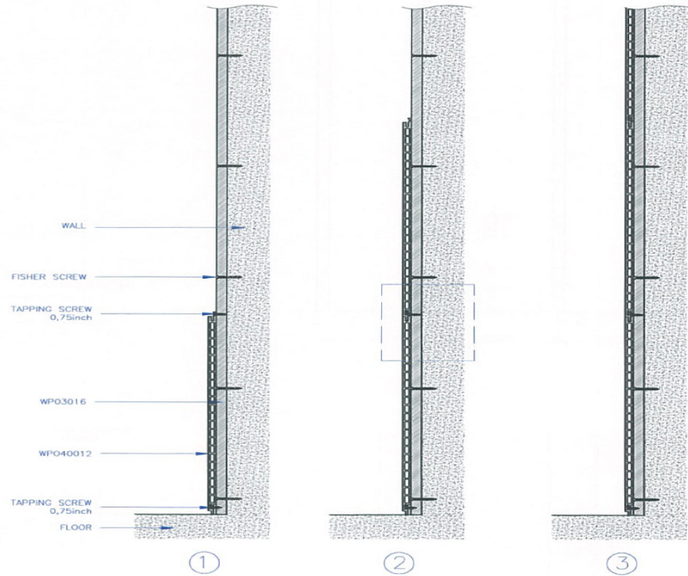
SIDE VIEW
