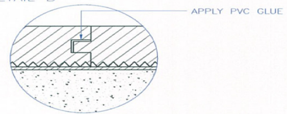
DETAIL B
