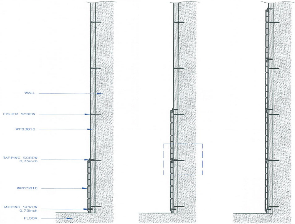
SIDE VIEW
