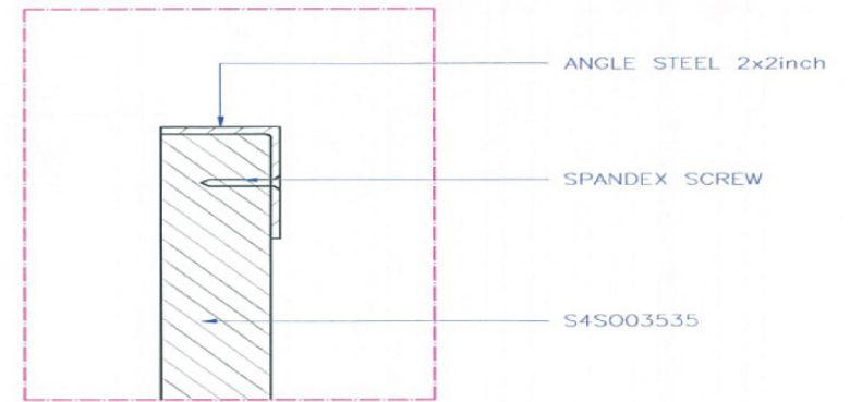
DETAIL A
