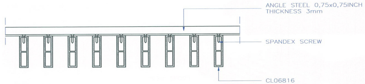
FRONT VIEW
