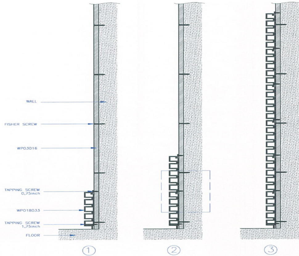
SIDE VIEW
