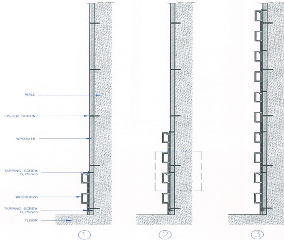
SIDE VIEW
