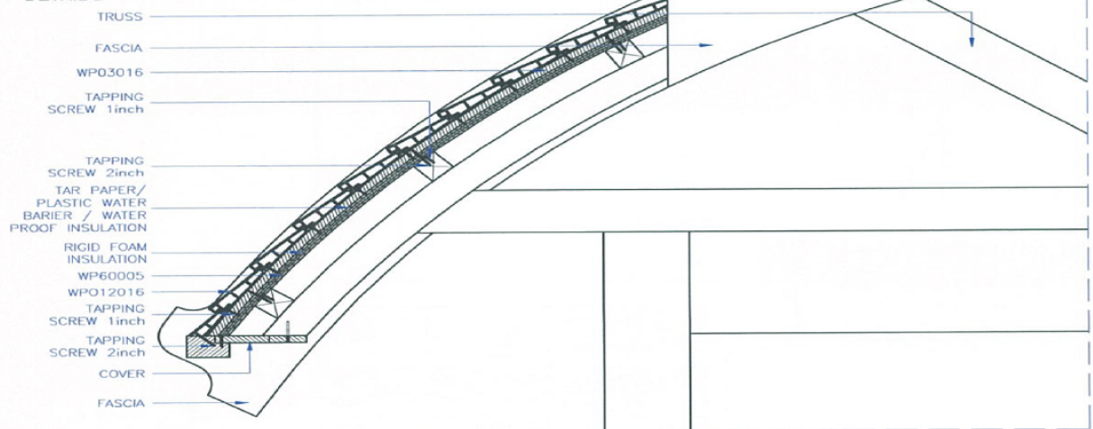
DETAIL B
