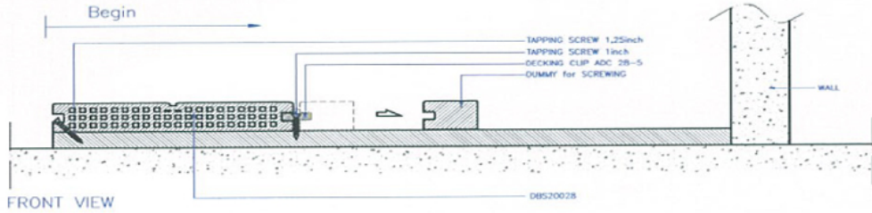
FRONT VIEW
