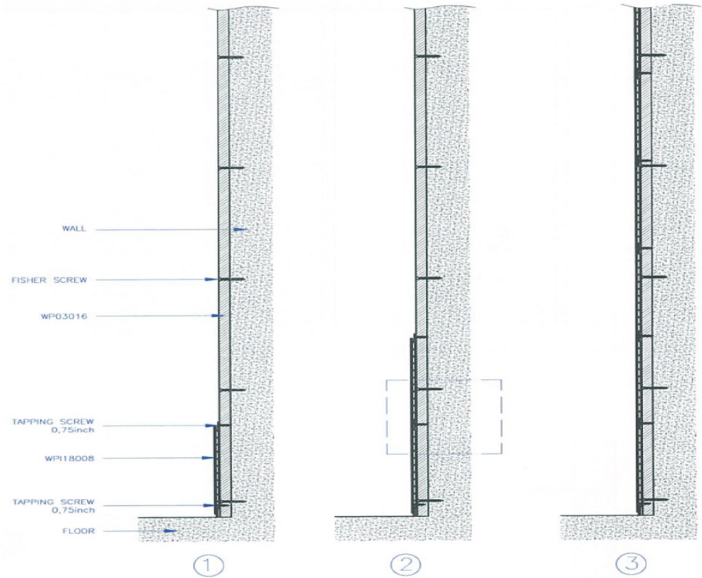
SIDE VIEW
