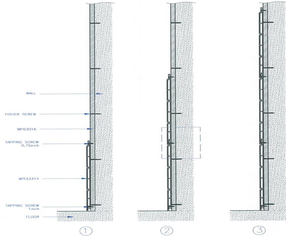
SIDE VIEW
