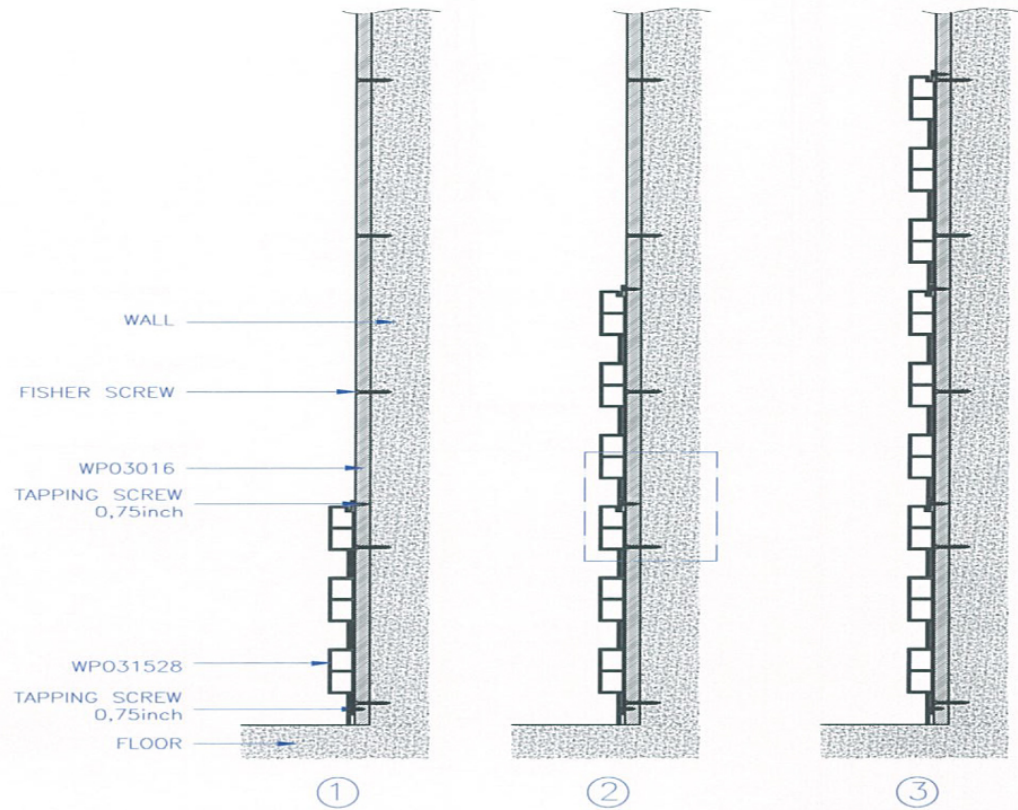
SIDE VIEW
