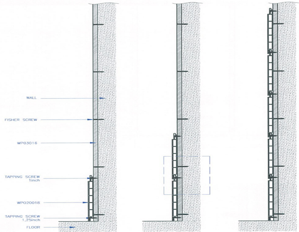
SIDE VIEW
