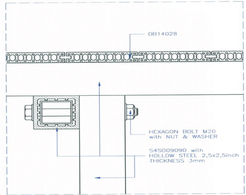
DETAIL A
