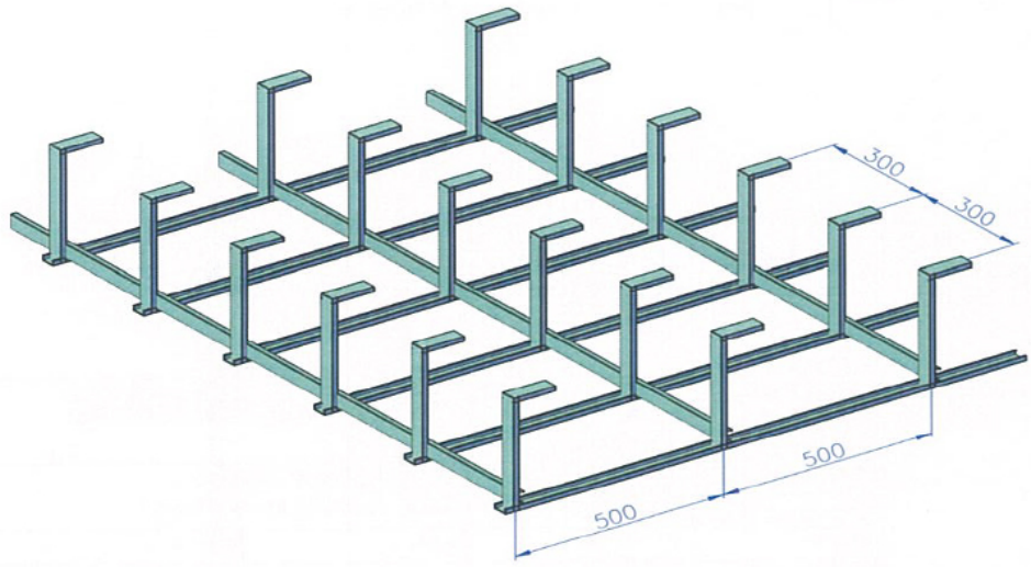
ECAFURING LAYOUT
