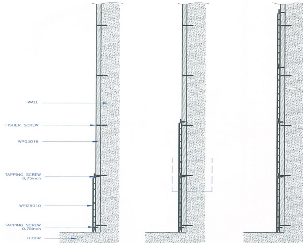
SIDE VIEW
