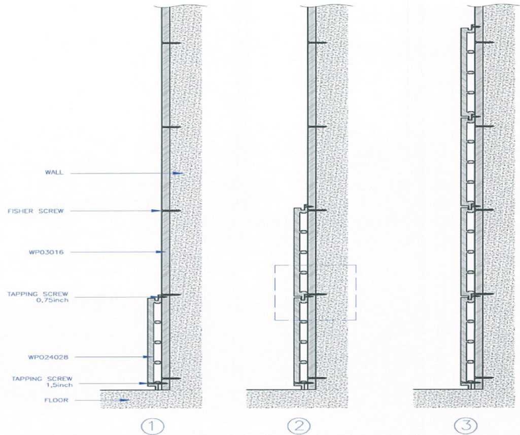
SIDE VIEW
