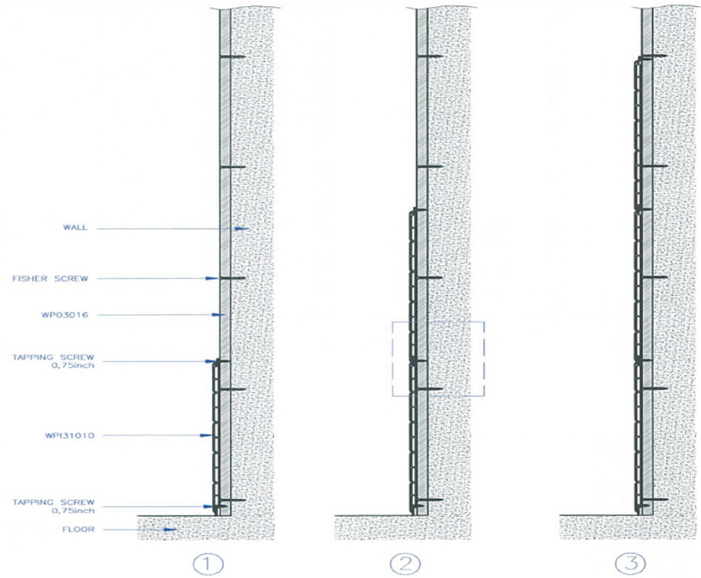
SIDE VIEW
