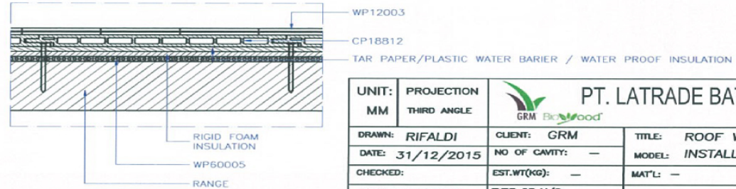
DETAIL B
