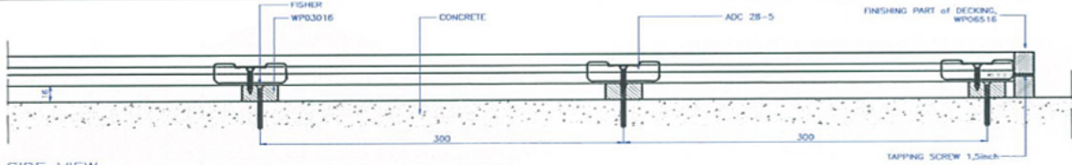
SIDE VIEW
