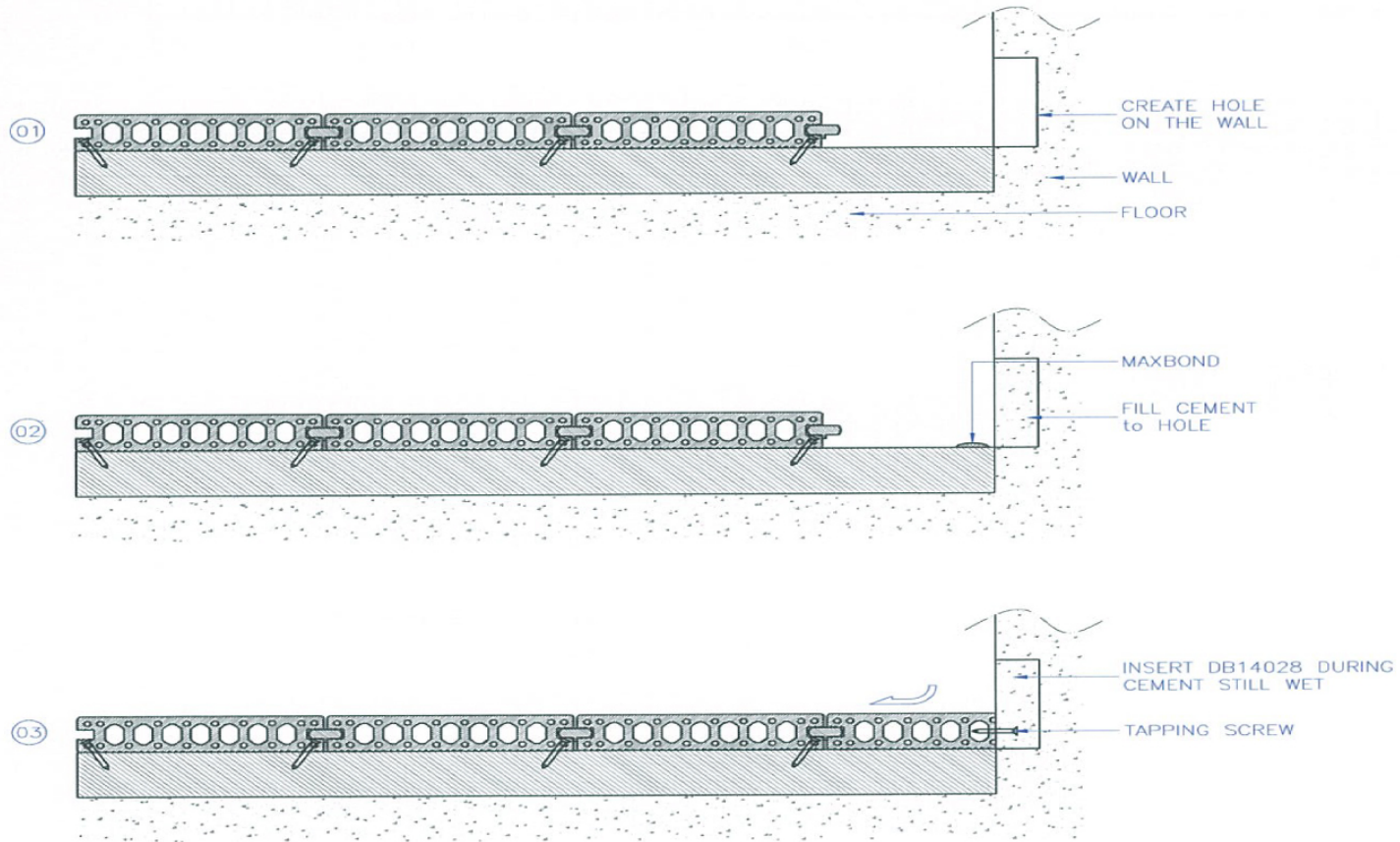
FRONT VIEW
