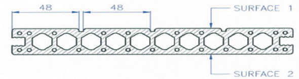
SURFACE 2
