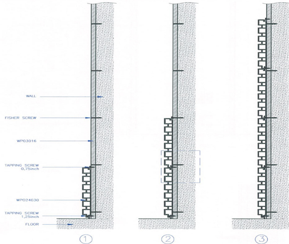
SIDE VIEW
