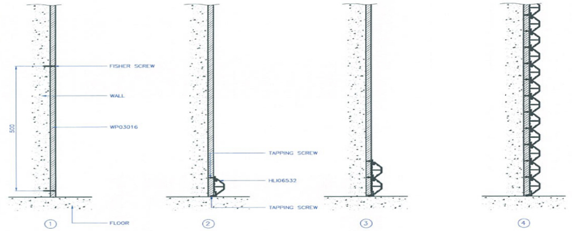
SIDE VIEW
