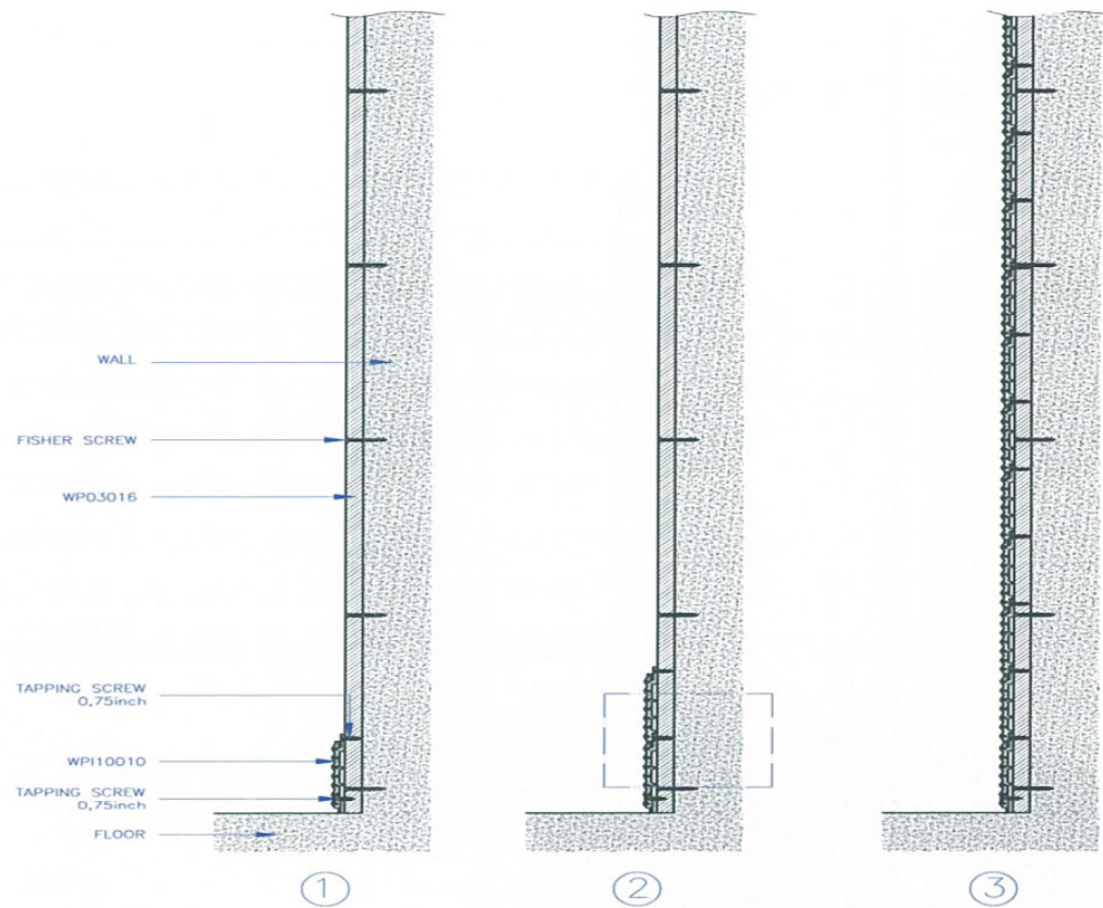
SIDE VIEW
