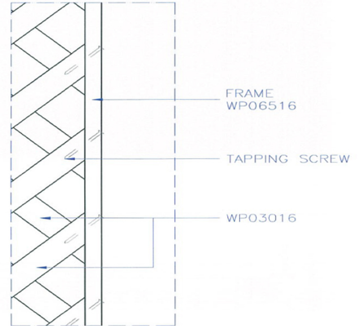
DETAIL A
