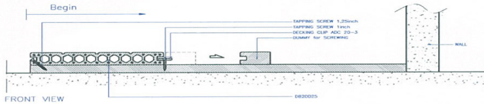
FRONT VIEW
