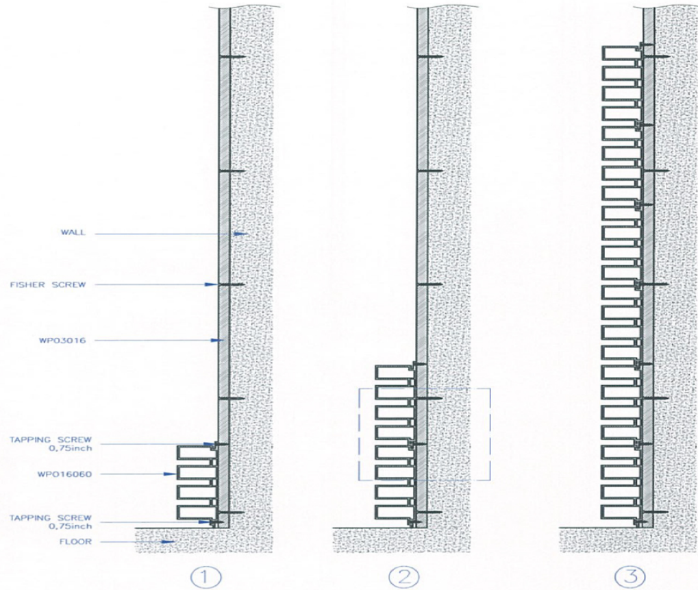
SIDE VIEW
