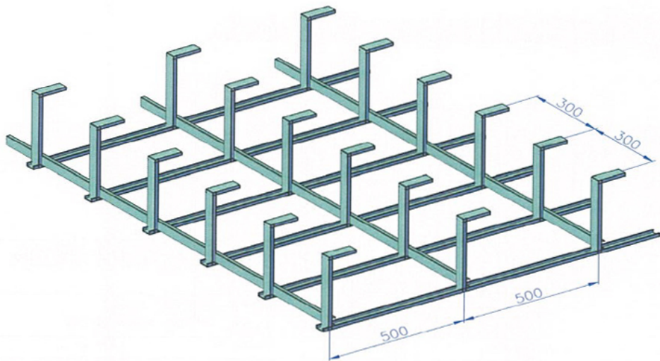
ECAFURING LAYOUT
