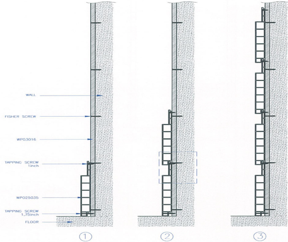
SIDE VIEW
