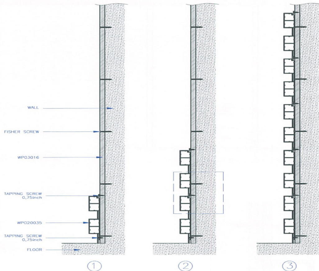
SIDE VIEW
