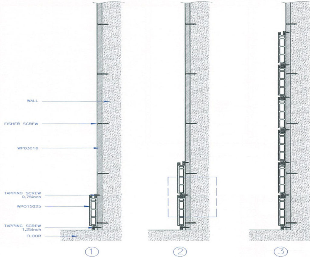
SIDE VIEW
