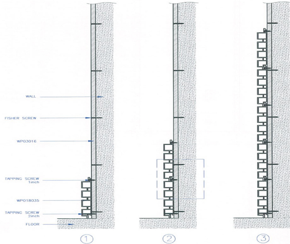
SIDE VIEW
